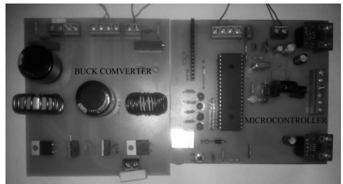
Fig. 6. Physical implementation of buck converter with microcontroller
