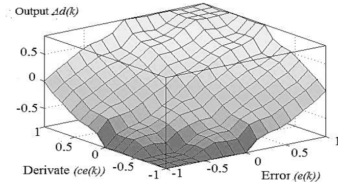
Fig. 4. Fuzzy levels for output signal versus e and ce for triangular type membership function.
