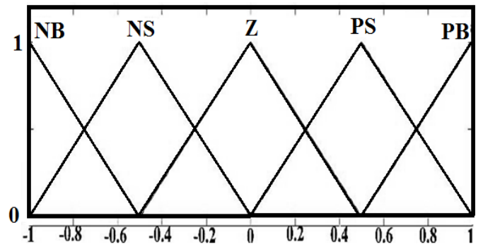
Fig. 3. Triangular type membership functions for e and ce
