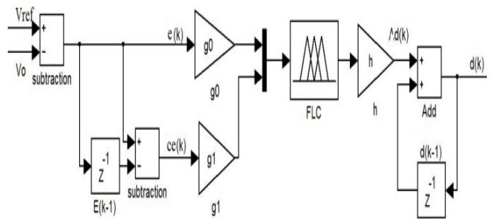
Fig. 2. Schematic diagram of fuzzy logic controller with gains and one integrator in the output
