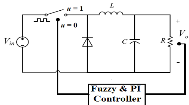
Fig. 1. The schematic of buck converter controllers
