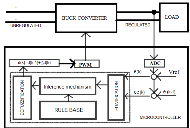
Fig.5. FLC in close loop for buck converter.
